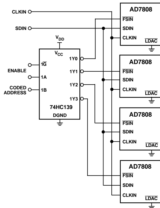
Figure 42. Decoding Multiple AD7808s Using the \overline{FSIN} Pin
